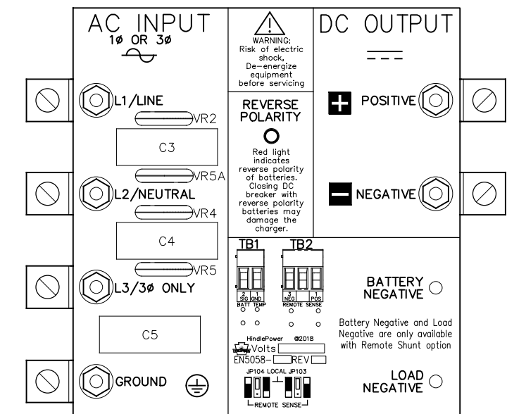
MOV PC BOARD (A9)
