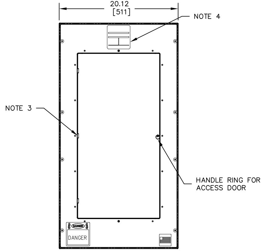
FRONT VIEW
