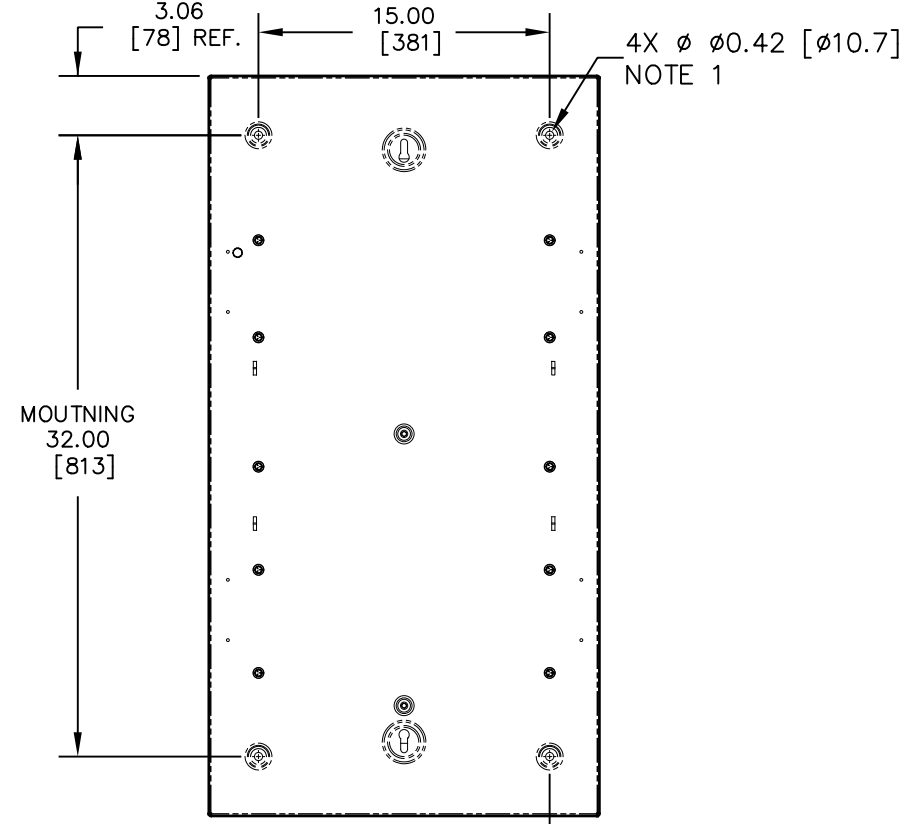
REAR VIEW
